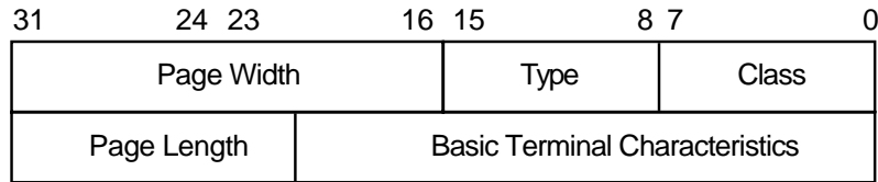
Figure 5–7 Set Mode and Set Characteristics Buffers
