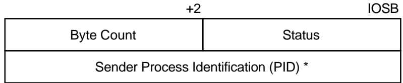
Figure 4–8 IOSB Contents—Read Function
