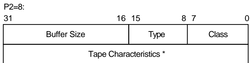
Figure 3–3 Sense Mode P1 Buffer
