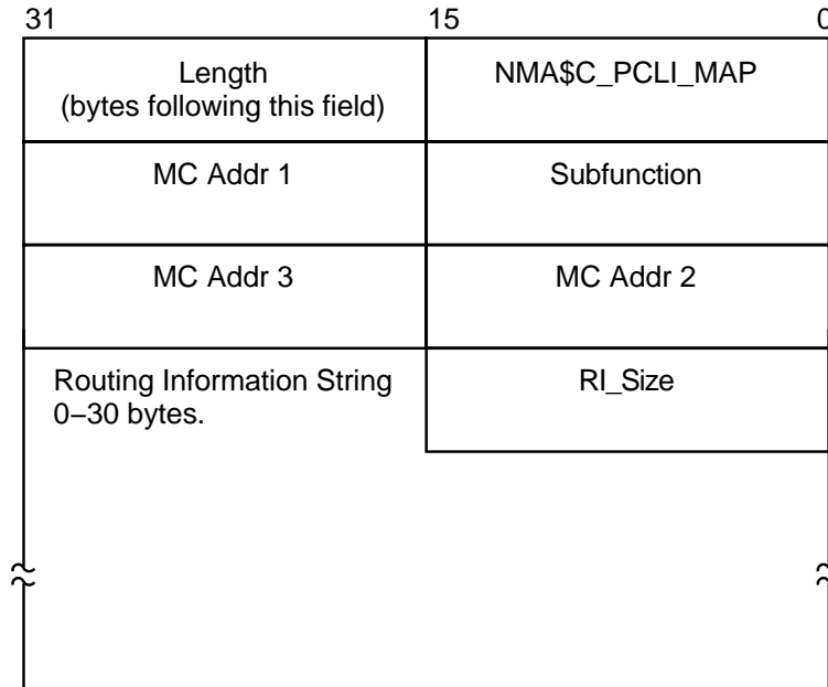
Figure 9-25 Format of the IO$M_ROUTE P2 Buffer (Alpha Only)
