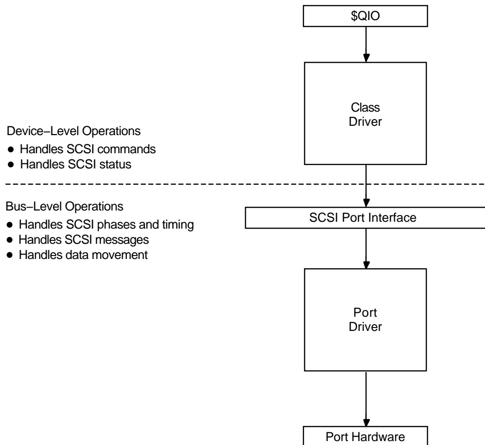
Figure 8-1 OpenVMS SCSI Class/Port Interface
