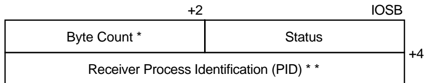
Figure 4–9 IOSB Contents—Write Function
