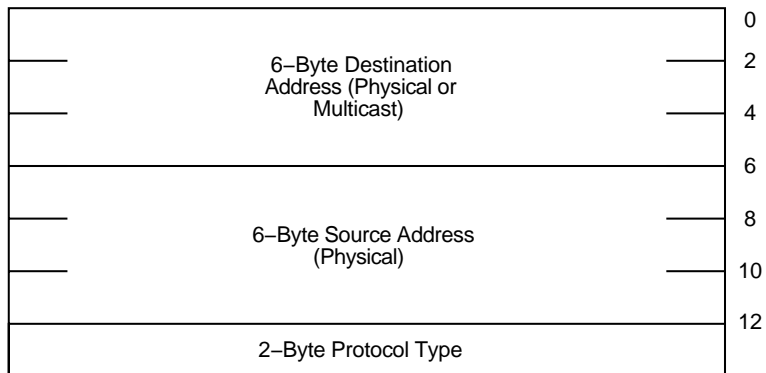
Figure 9–21 Read Function P5 Buffer
