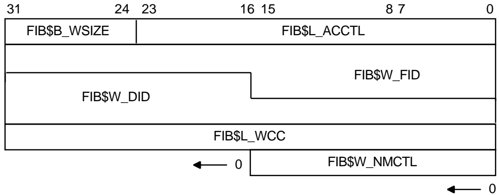
Figure 1-5 Typical Short FIB
