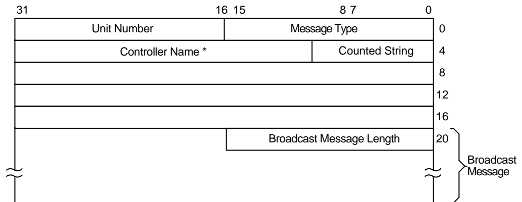
Figure 5-2 Terminal Mailbox Message Format
