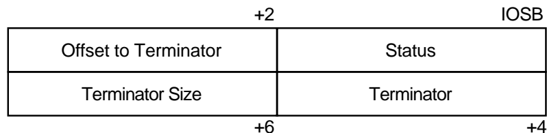
Figure 5–14 IOSB Contents—Read Function
