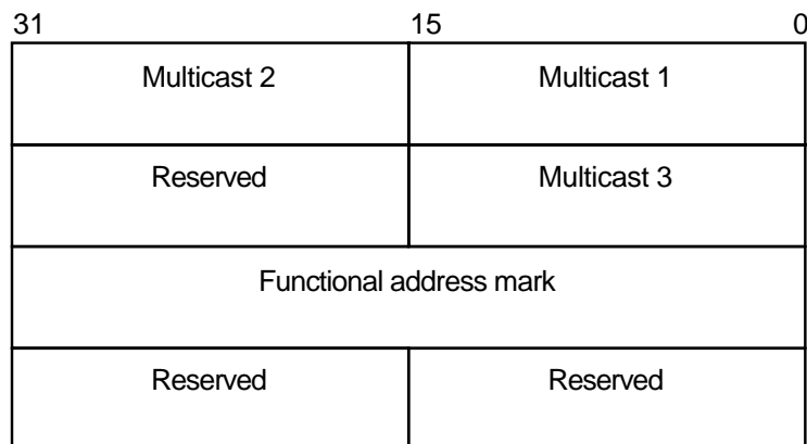
Figure 9–28 Format of IO$M_SHOW_MAP P2 Buffer (Alpha Only)
