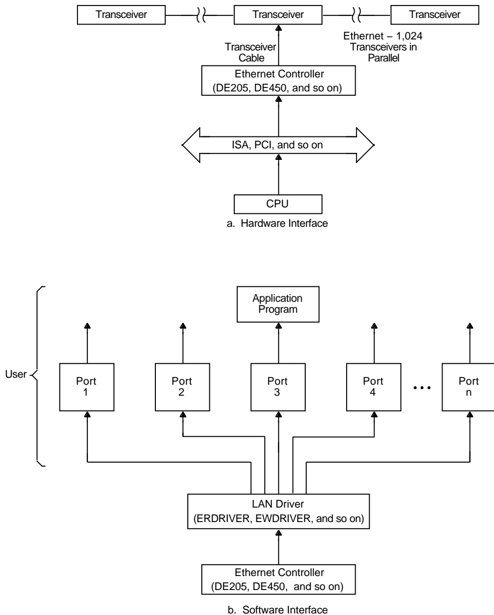
Figure 9–2 Typical Ethernet Configuration
